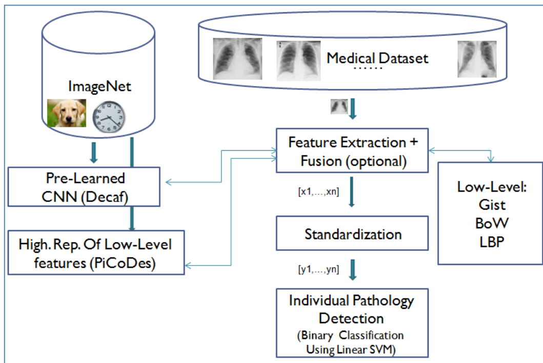
Figure 2: Algorithm flowchart.
