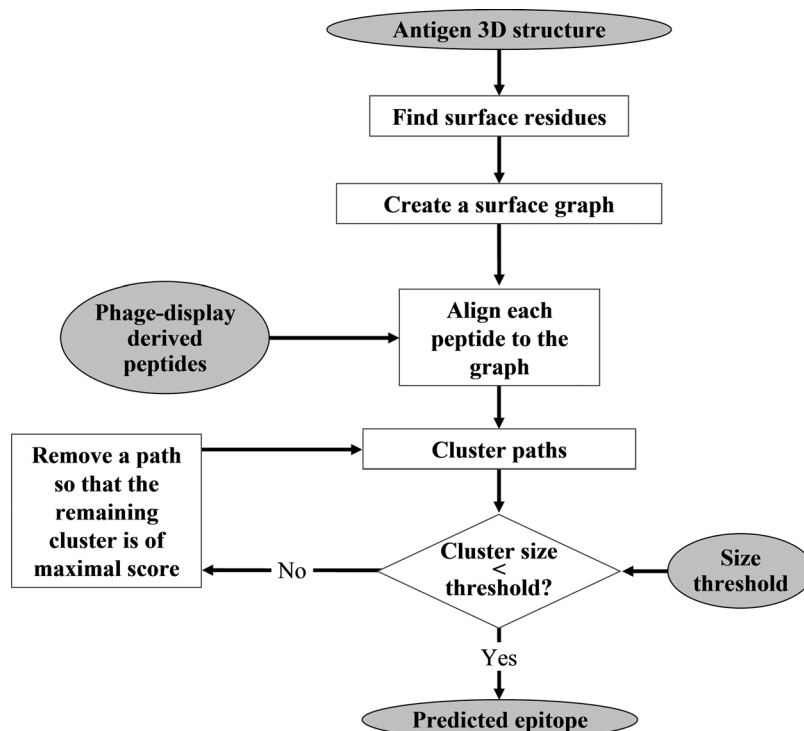
Figure 1. A schematic flowchart of the PepSurf algorithm.
