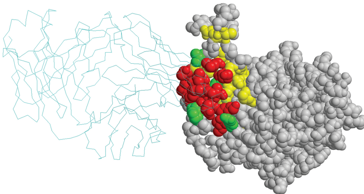
Figure 2. The prediction obtained by the PepSurf algorithm for the 17b–gp120 complex (PDB identifier 1G9M). The gp120 and 17b antibody are shown as a space-filling and backbone models, respectively. Residues successfully predicted are colored red, residues erroneously inferred to be part of the epitope are colored green, and genuine epitope residues not predicted are colored yellow.
