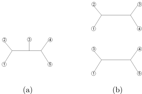
Figure 2: (a) A phylogenetic tree over five leaves. (b) Two quartets compatible with the tree on the left.
