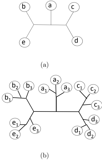
Figure 4: (a) A tree T' on taxa set \mathcal{X}^* = \{a, b, c, d, e\} . (b) The tree T' on taxa set \mathcal{X} after replacing each leaf with its k copies ( k = 3 in this example).
