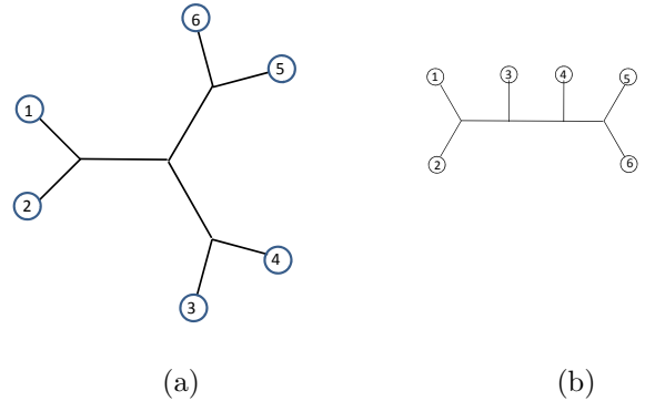
Figure 5: (a) The 6-flower tree. (b) The 6-caterpillar tree [12|3|4|56] .
