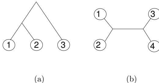
Figure 1: In a rooted setting, a rooted triplet is the smallest informative tree versus an unrooted quartet in the unrooted setting. (a) - a rooted triplet tree [12|3]. (b) - an unrooted quartet tree [12|34].
