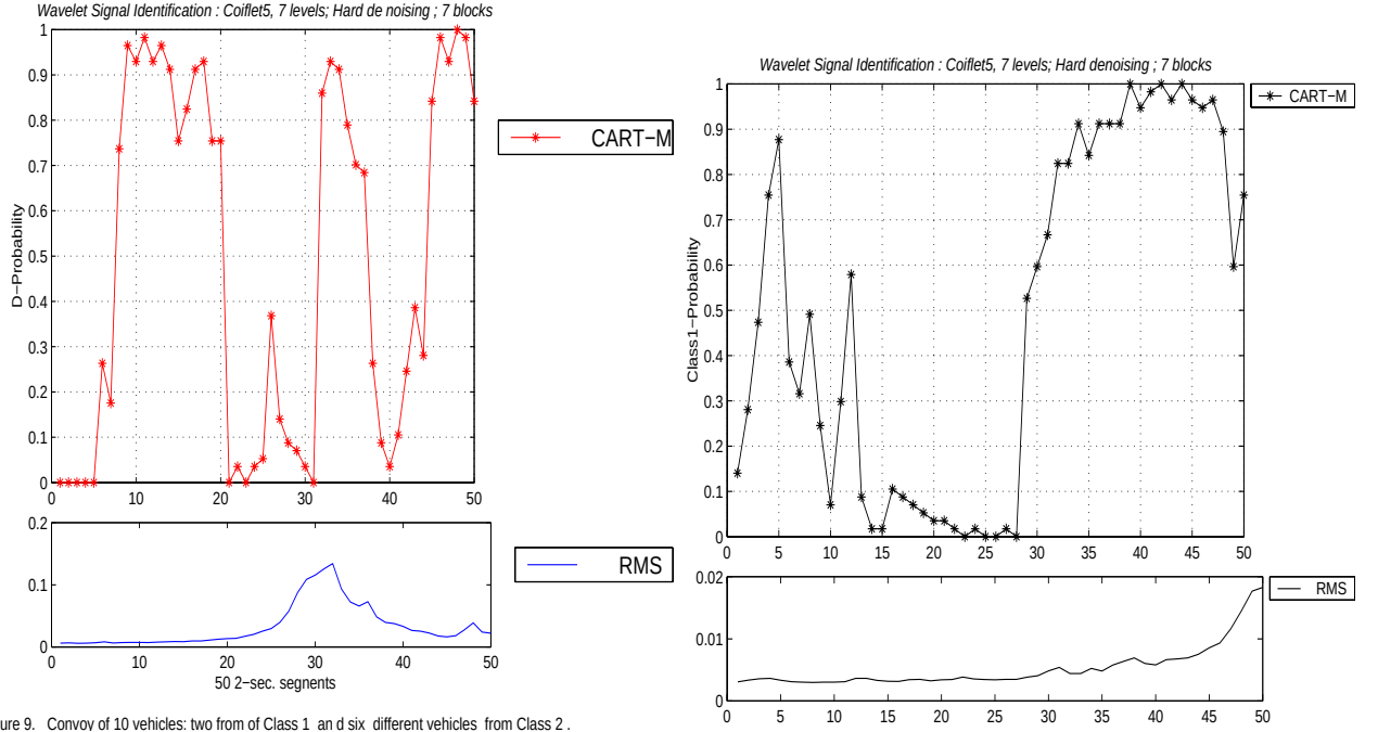
Figure 9. Convoy of 10 vehicles: two from of Class 1 and six different vehicles from Class 2.
