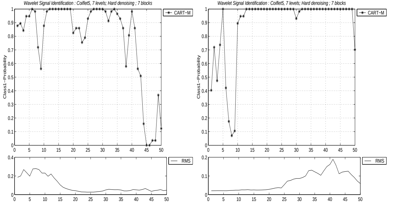
Figure 8: A vehicle from Class 1 is moving away from the receiver up a a distance of 1000 meters (left top picture). The vehicle approached the receiver from 900 meters distance at 40 km/h. Bottom pictures depict the RMS of each 2-second signal. They all traveled on ground road. The following parameters were used: Coiflet5 wavelets, 7 blocks, modified CART classifier and every 2 seconds a decision was made.
