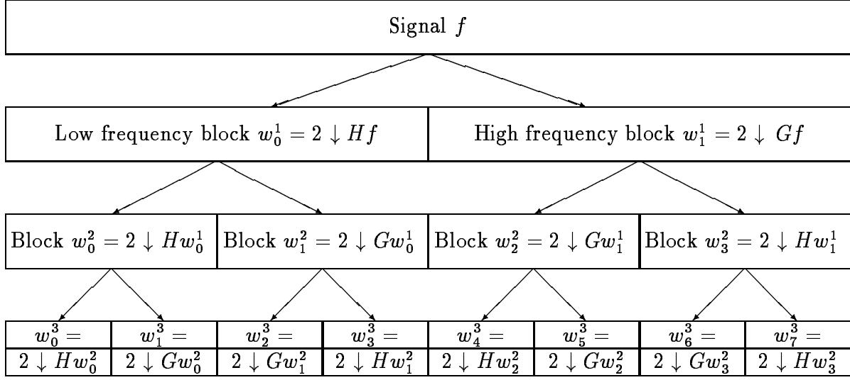
Figure 11: Three levels of wavelet packet decomposition.
