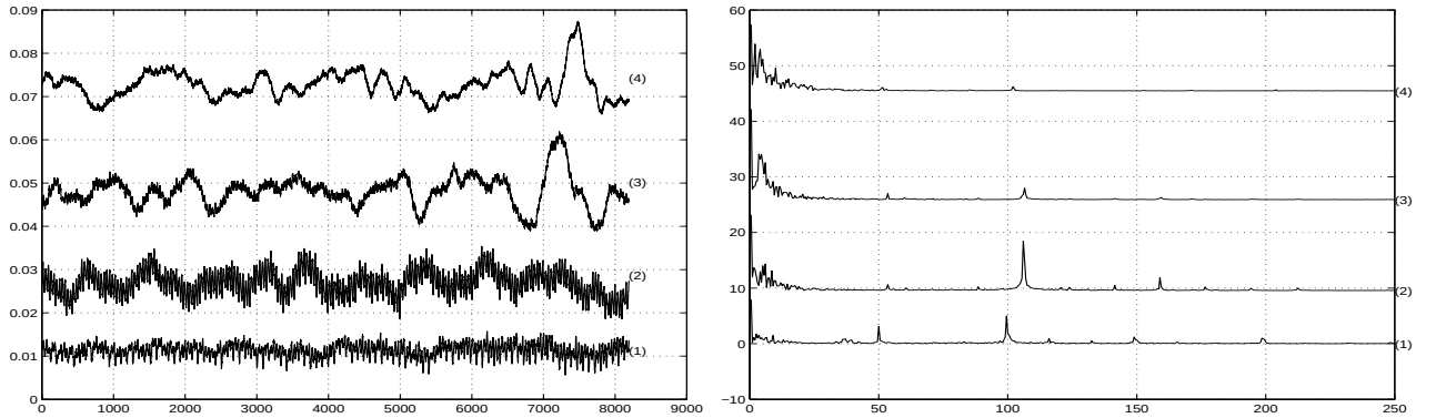
Figure 2: Left picture: sections of class C^1 -signal recorded at different conditions: line 1—the vehicle is approaching the receiver; line 2—passing by the receiver; line 3—moving away from the receiver at a moderate speed; line 4—the same but far away from the receiver. Right picture: portions of the Fourier transforms of the signals shown in the left picture.
