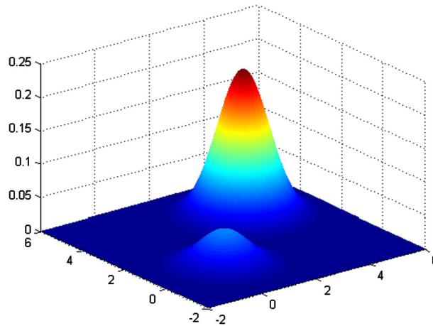
Fig. 2. The analytical stationary distribution.
