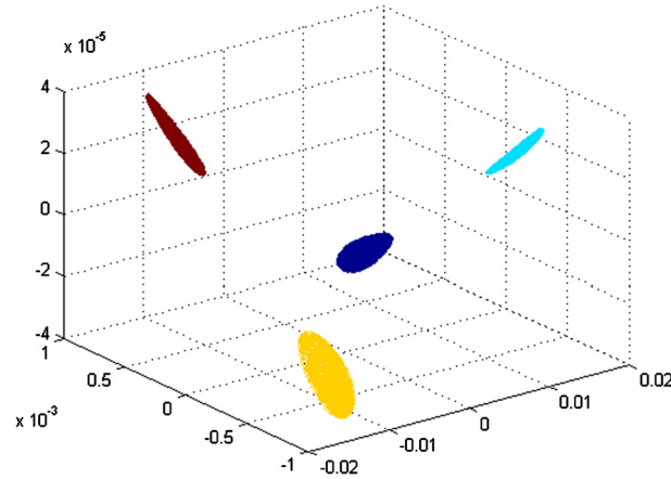
Fig. 5. The embedding of data points sampled from a four-well potential.
