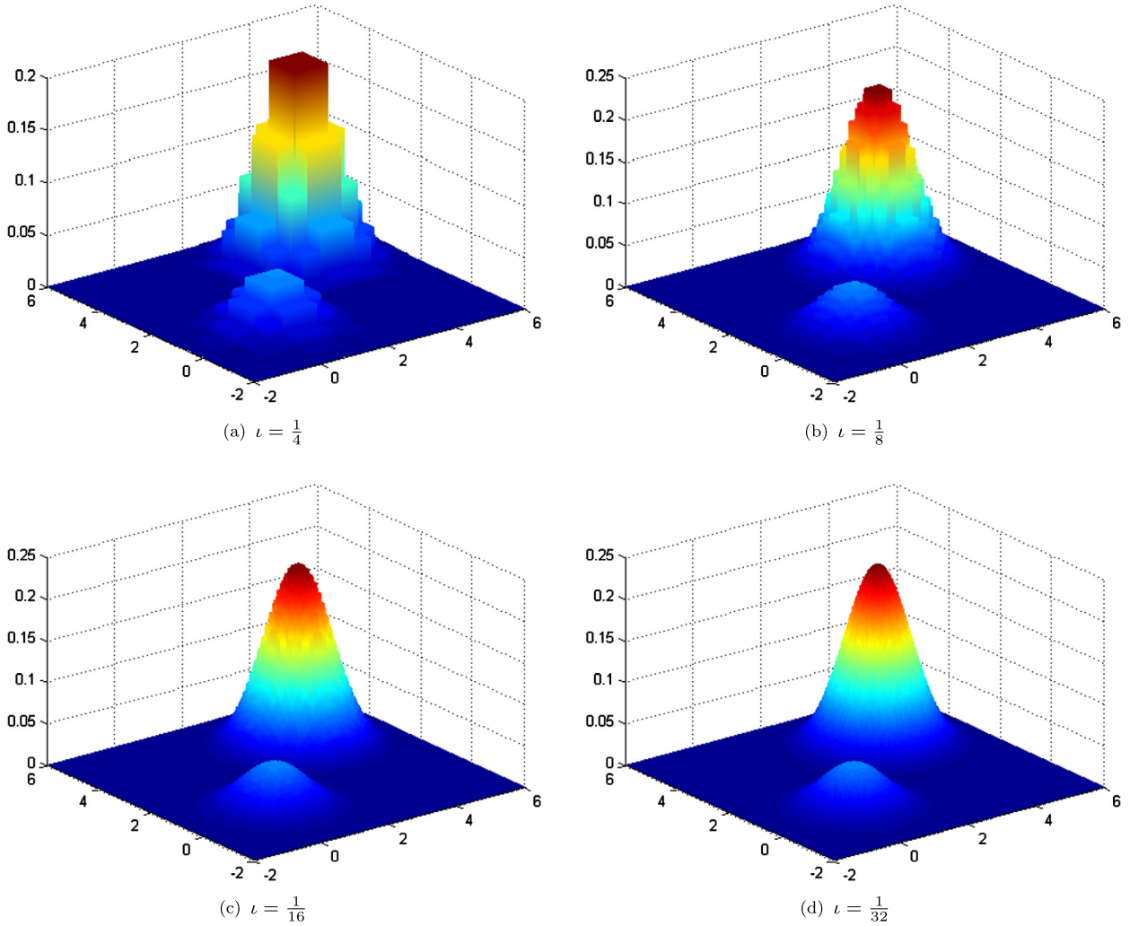
Fig. 3. Comparing between the discrete stationary distribution and the analytical stationary distribution as a function of \epsilon . (a) \epsilon = \frac{1}{4} . (b) \epsilon = \frac{1}{8} . (c) \epsilon = \frac{1}{16} . (d) \epsilon = \frac{1}{32} .
