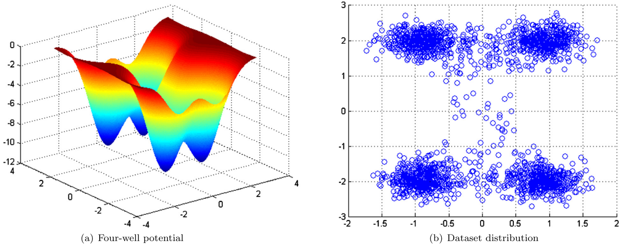
Fig. 4. (a) Four-well potential. (b) Data point distribution that corresponds to the given potential.
