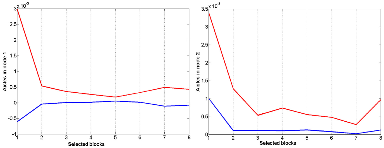
Fig. 14. Examples of Aisles in two different CART nodes. X-axes: indices k = 1, \dots, 8 of the coordinates of the row vectors. Upper lines: \bar{m}^k + 2\bar{s}^k . Lower lines: \bar{m}^k - 2\bar{s}^k .
