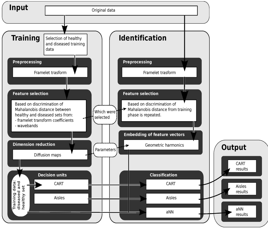
Fig. 5. Processing pipeline.
