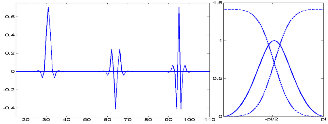
Fig. 7. Left: left-to-right impulse responses of the filters: \mathbf{h}^0 \rightarrow \mathbf{h}^1 \rightarrow \mathbf{h}^2 . Right: magnitude responses of \mathbf{h}^0 and \mathbf{h}^2 (dashed lines) and \mathbf{h}^1 (solid line).
