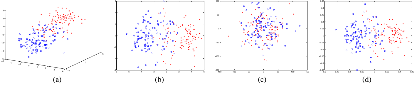
Figure 1: This figure demonstrates the importance of feature selection in the unsupervised setting, and that even though our algorithms and PCA use similar optimization functions, they are very different in their capabilities of dealing with irrelevant variables: (a) Three relevant dimensions out of 203. The rest of the dimensions are similar but were permuted to remove any class membership information; (b) The first 2 principle components of only the 3 relevant dimensions; (c) PCA of the whole 203 dimensions; (d) The results of applying PCA after weighting according to the \alpha weights recovered by Algo. 1.
