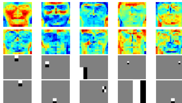
Figure 3: Top two rows show the first 10 principle components of the wavelets weighted by Algo. 2 on the YALE dataset. Bottom rows show the first 10 wavelet features picked by Algo. 2 on the same experiment.
