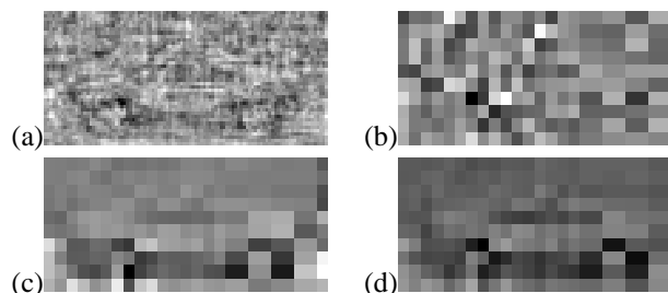
Figure 4: Template for car detection learned via SVM from four different feature sets. (a) histogram equalized gray levels (b) Haar wavelets (c) Algo. 2 on Haar wavelets (d) Algo. 3 on Haar wavelets.
