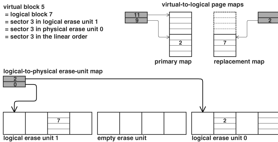
Fig. 2. An example of the FTL mapping structures. The system in the figure maps two logical erase units onto three physical units. Each erase unit contains four sectors. Sectors that contain page maps contain four mappings each. Pointers represented as gray rectangles are stored in RAM. The virtual-to-logical page maps, shown on the top right, are not contiguous so a map in RAM maps their sectors. Normally, the first sectors in the primary map reside in RAM as well. The replacement map contains only one sector; not every primary map sector must have a replacement. The illustration of the entire device on the bottom also shows the page-map sectors. In the mapping of virtual block 5, the replacement map entry is used, because it is not free (all 1's).
