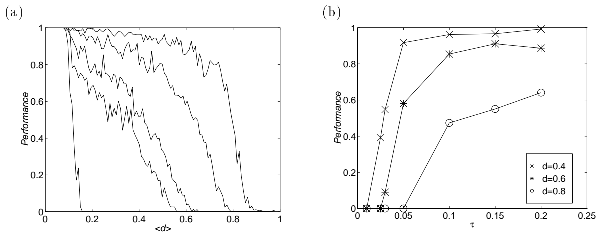
Figure 3: (a) Performance versus deletion for different compensation rates. \tau is increased from left to right, with values 0.01, 0.025, 0.03, 0.05, 0.1. \Delta d = 0.009 . (b) Performance versus \tau for fixed d values.
