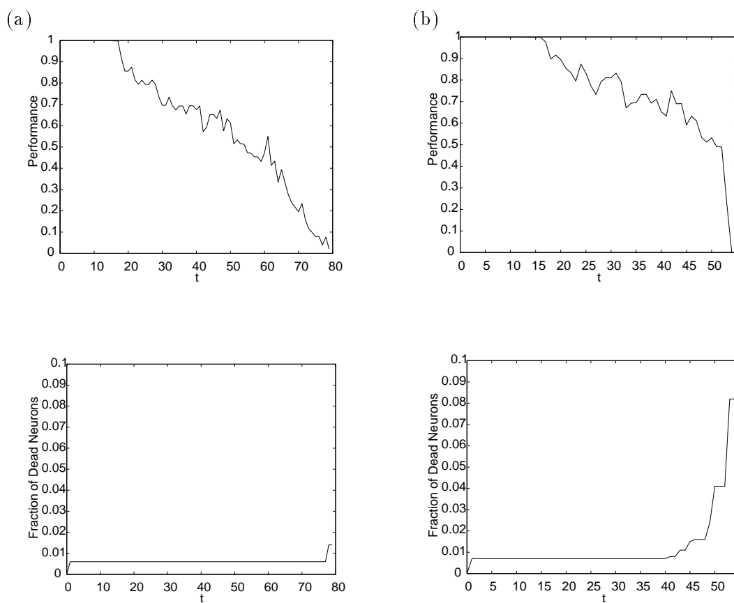
Figure 5: Performance versus time with (a) a low viability threshold ( VT = 0.2 ) and (b) a high viability threshold ( VT = 0.5 ). \tau = 0.02 and the rest of the simulation parameters are as in Figure 7. The bottom figures trace the fraction of dead neurons as a function of time. Neuronal damage is traced until complete performance collapse (the patient’s ‘death’), i.e., zero overlap.
