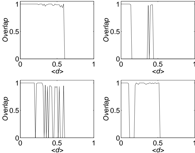
Figure 4: Overlaps of individual patterns. The simulation parameters were \Delta d = 0.015 and \tau = 0.05 .
