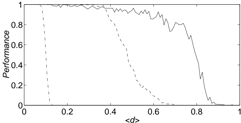
Figure 2: Performance versus deletion for a network that runs the local Willshaw-compensation algorithm (8). The result, presented by a solid line, is compared with the performance of local TSA conservation ( c_i = 1/w_i , dashed curve) and no compensation ( c_i = 1 , dot-dashed curve) methods. The simulation parameters were N = 1500 , M = 75 , p = 0.05 , \tau = 0.1 , \Delta d = 0.009 .
