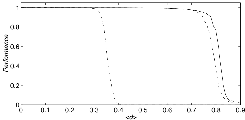
Figure 1: Performance versus deletion for a network that runs the local TF-compensation algorithm via (4) and (6). The result, presented by a solid line, is compared with the performance of local TSA conserving method ( c_i = 1/w_i , dashed curve) and no compensation ( c_i = 1 , dot-dashed curve). The simulation parameters were N = 1000, M = 100, p = 0.1, \tau = 0.25, \Delta d = 0.01 .
