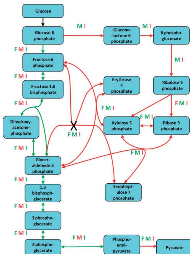
Fig. 4. An example flux distribution predicted by IOMA following the knockout of talB ( Transaldolase B ). The network shows E.coli 's glycolysis and PPP. Green (red) edges represent a measured increase (decrease) of flux between the wild-type and knockout strains. The letters F, M and I, represent predictions made by FBA, MOMA and IOMA, respectively, with green (red), representing a predicted increase (decrease) in flux. Predictions of no significant change in flux are not shown. As evident, IOMA correctly predicts the measured pattern of increased flux throughout glycolysis and decreased flux throughout the PPP pathways, with only two mismatches, while FBA and MOMA perform significantly worse.
