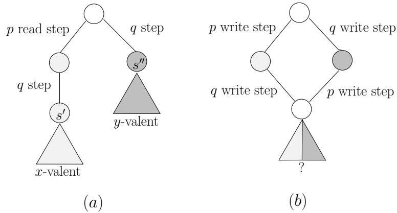
Figure 1: The decision steps cases.
