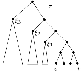
Figure 8. The tree \tau . If a subtree \tau(\xi_1) is part of the output for a vertex v , all subtrees that are left children of nodes on the path from \xi_1 to the root are also part of that output.
