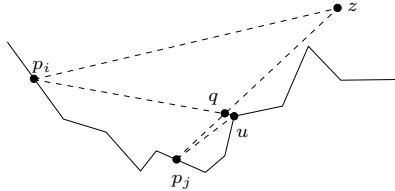
Figure 15. Points z \in W_j^r to the right of u are visible from p_i .
