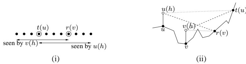
Figure 13. (i) Proof of the ‘if’ part. (ii) The case r(v) < t(u) .
