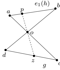
Figure 11. The relation between the point p(s, h) on e_1(h) and z_g(s) on g . Here o is the pivot vertex of T .
