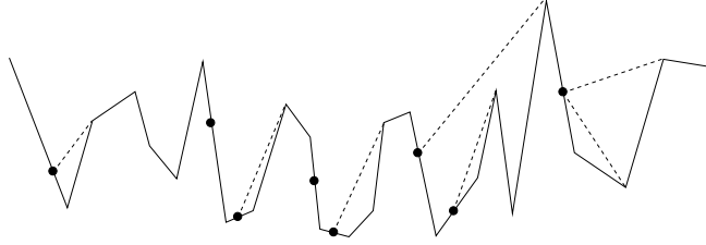
Figure 2. Some pairs of \Pi(P, V) .
