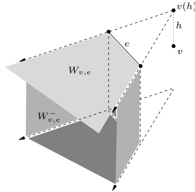
Figure 16. The truncated wedge W_{v,e} and the prism W_{v,e}^- .
