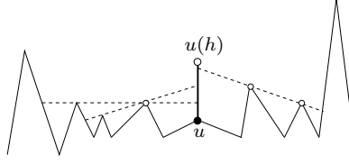
Figure 6. The critical heights over u .
