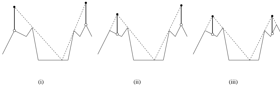
Figure 1. The three versions of the problem in \mathbb{R}^2 : (i) discrete, (ii) semi-discrete, and (iii) continuous.
