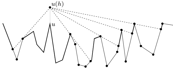
Figure 5. The visible portions of T from u(h) , and the set P(u, h) (highlighted along T ).
