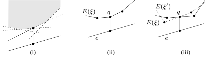
Figure 7. (i) The shortest vertical distance from an edge of T to the corresponding upper envelope. (ii) The shortest vertical distance from e to the envelope is attained at a vertex of a single subenvelope. (iii) The shortest distance is attained at an intersection point between two subenvelopes.
