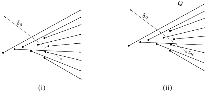
Figure 3. (i) The rays \gamma_p and a query ray \delta_q . (ii) The polygon Q .
