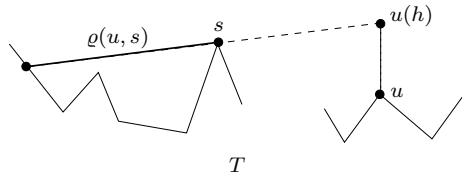
Figure 17. The segment \varrho(u, s) .
