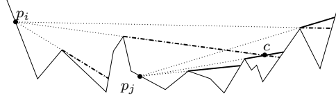
Figure 14. Two points p_i, p_j and their visibility polygons W_i and W_j . Only the right portions of these polygons are drawn. The portions \overline{W}_i, \overline{W}_j of the boundaries of these polygons that lie strictly above T are drawn as dashed-dotted and solid, respectively.
