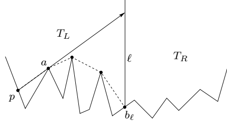
Figure 4. Constructing the rays \gamma_p from the shortest-path map from b_\ell .
