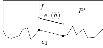
Figure 9. Creating a simple polygon P' from T and e_1(h) .
