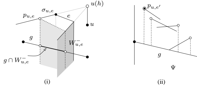
Figure 18. (i) Intersection of g and a prism W_{u,e}^- . (ii) The vertical strip \Psi and its intersection with the wedges W_{u,e}^- .
