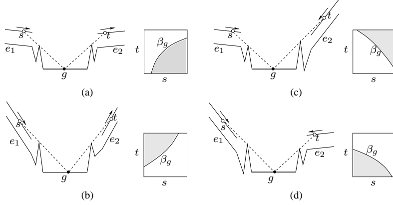
Figure 12. The four types of mutual visibility of an edge g from a pair of moving towers, and the corresponding st -regions where the entire g is guarded.
