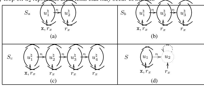
Fig. 2. (a),(b),(c) Examples of 2-valued structures representing linked-lists that are pointed to by program variable x , of length 2, 3, and 4, respectively. (d) S represents all lists that are pointed to by program variable x and that have at least two elements, including the lists represented by (a)-(c).
