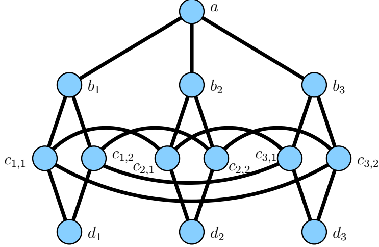
Figure 3: A diameter-3 sum equilibrium graph.
