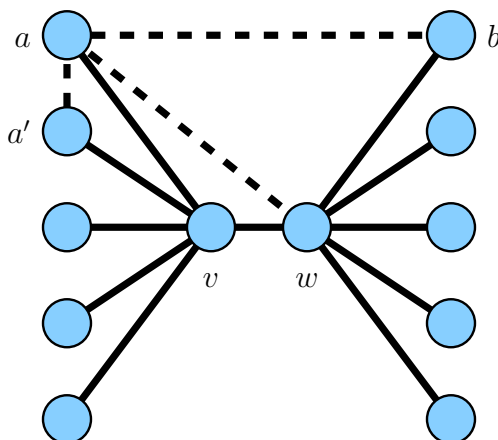
Figure 2: A tree of diameter 3 that is insertion-stable and hence in max equilibrium. There are three types of edges we might try to add, shown dashed: from a leaf a to a cousin leaf a' or to a distinct leaf b or to the other root w . None of these edges improves the local diameter of either endpoint.
