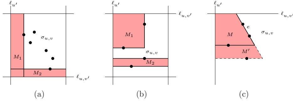
Figure 8: Anchored maximal R_{u,v} -empty rectangles (a) for upper quadrants, and (b) for lower quadrants. (c) The right trapezoid M' cannot be empty, if the slanted edge e also belongs to M .
