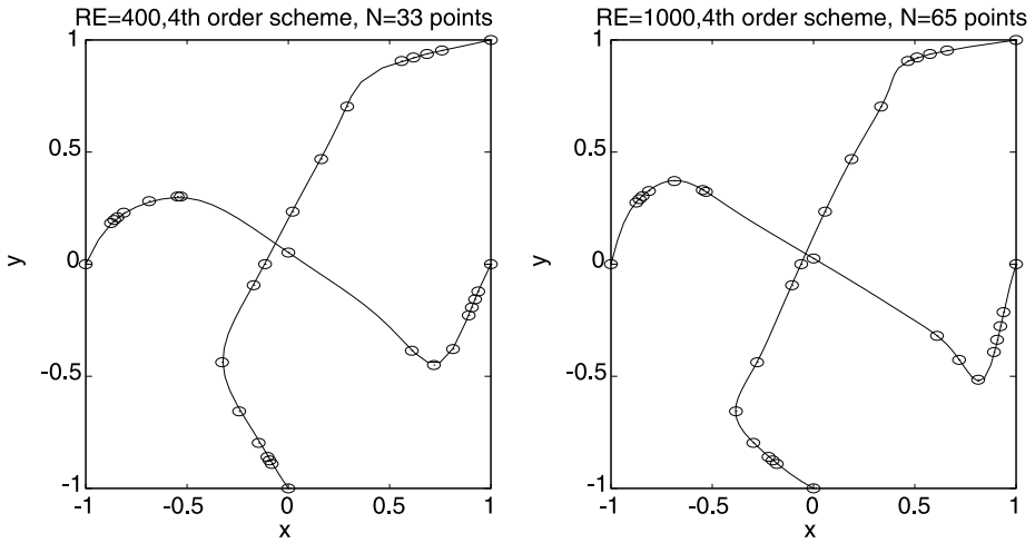
Fig. 1 Velocity components for the driven cavity problem. Left: Re = 400 , fourth-order scheme with N = 33 (solid line), [9] with N = 129 (circles). Right: Re = 1000 fourth-order scheme with N = 65 (solid line), [9] with N = 129 (circles)
