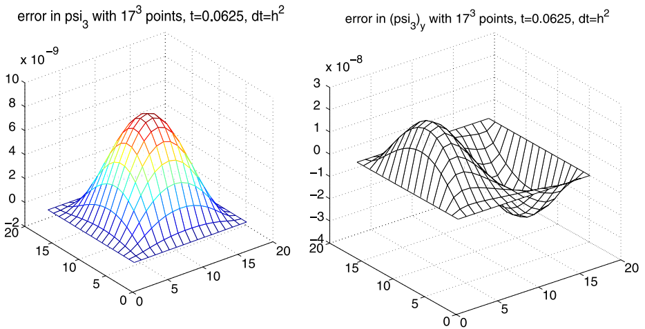
Fig. 3 Navier-Stokes: Errors in \psi_3 and (\psi_3)_y for N = 17 , t = 0.0625 , \Delta t = h^2 . The exact solution is \psi^T(\mathbf{x}, t) = -\frac{1}{4}e^{-t}(z^4, x^4, y^4)
