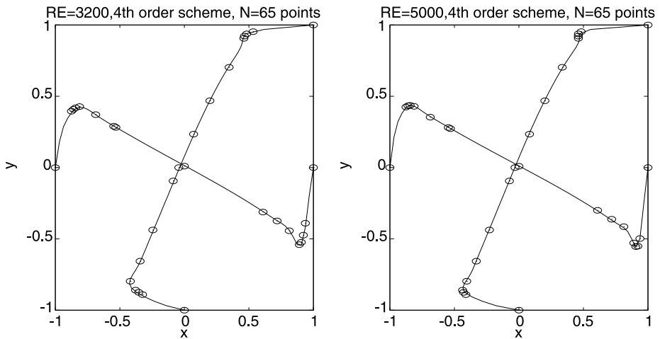
Fig. 2 Velocity components for the driven cavity problem. Left: Re = 3200 , fourth-order scheme with N = 65 (solid line), [9] with N = 129 (circles). Right: Re = 5000 fourth-order scheme with N = 65 (solid line), [9] with N = 257 (circles)
