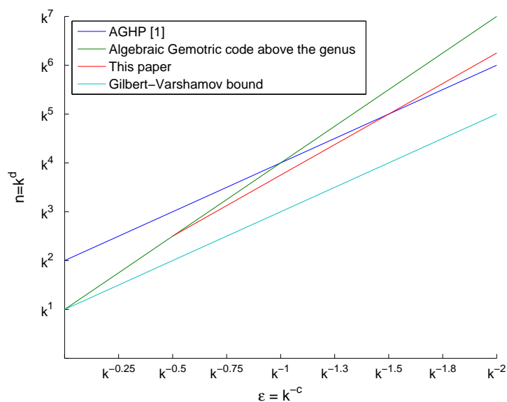
Figure 1: Constructions of \epsilon -biased sets for \epsilon = k^{-c}
