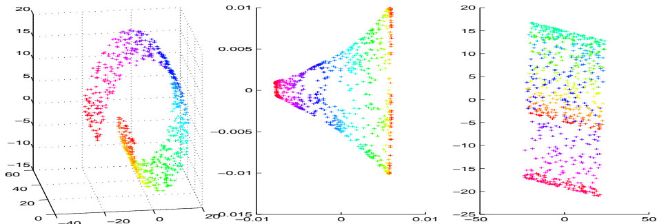
Figure 1: “Swiss roll”, 2-dimensional Laplacian representation, and PCA representation, left to right. For the purposes of illustration we compare a spectral 2-dimensional representation of the “swiss roll” to principal component analysis. PCA is limited to projections and therefore cannot produce a good representation of non-linear data.
