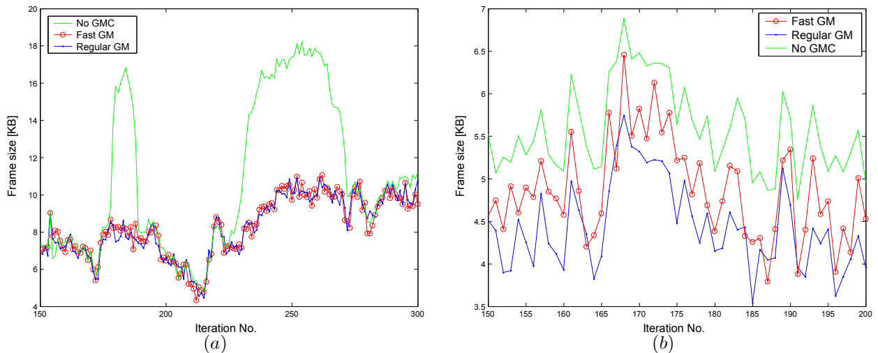
Fig. 7. MPEG4 Compression results for sub-sequences within the sequences in Fig. 6. (a) In this subsequence of Stefan, a global motion occurs as the player rushes to the net. Using GME results in a significant reduction in the encoded frame size. (b) A subsequence of Fig. 6.b, due to significant occlusion in the scene the improvement caused of the Fast GM is 10% less than the regular GM, but the computational complexity is less by 20 fold.
