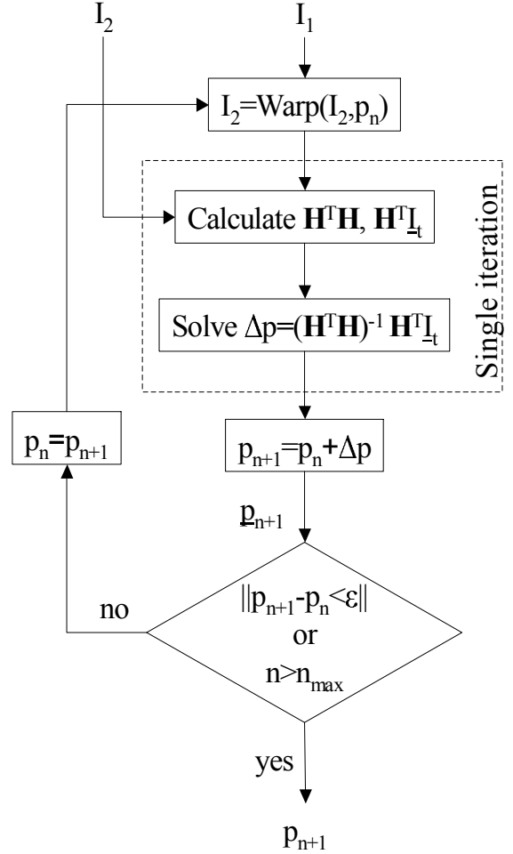
Fig. 1. Block diagram of the basic and iterative GM formulations. For n = 0 , p_0 is given as an initial guess and \Delta p is the iterative update after each iteration.
