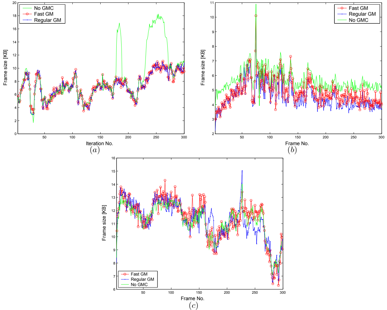
Fig. 6. MPEG4 Compression results using the Fast GM, regular GM and non-GMC compression modes for (a) Stefan, (b) Coastguard and (c) Mobile sequences. The sequences were encoded using Q = 31 , thus the compression results are directly related to the GMC efficiency. The Fast GM provides compression results very similar to the regular GM, while utilizing 20 times less computational complexity.
