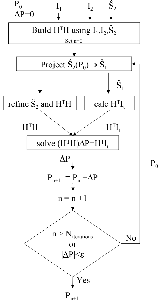
Fig. 4. A flow chart of the SIGM iterative image registration. The flow chart follows the procedure described in section III-C.
