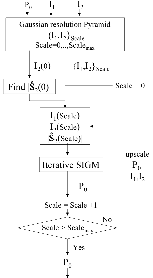
Fig. 3. SIGM multiscale image registration flow chart. The scheme utilizes the iterative registration presented in Fig. 4.
