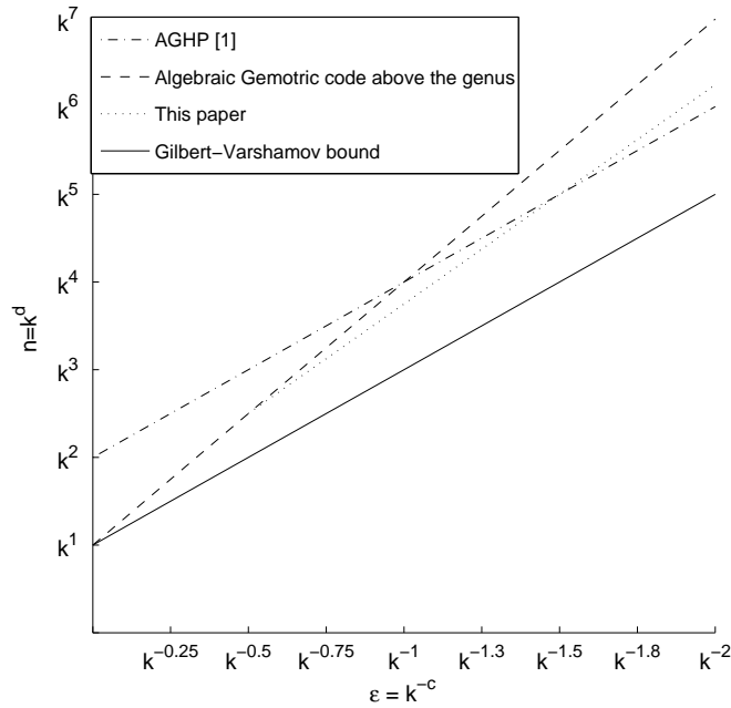
Figure 1: Constructions of \epsilon -biased sets for \epsilon = k^{-c}
