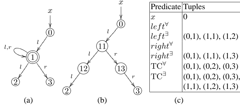
Fig. 9. (a) Abstract state S_3 , (b) a concrete state C_2 s.t. (S_3, C_2) \in \gamma that demonstrate the problem with the improved translation (c) \widehat{S}_3
