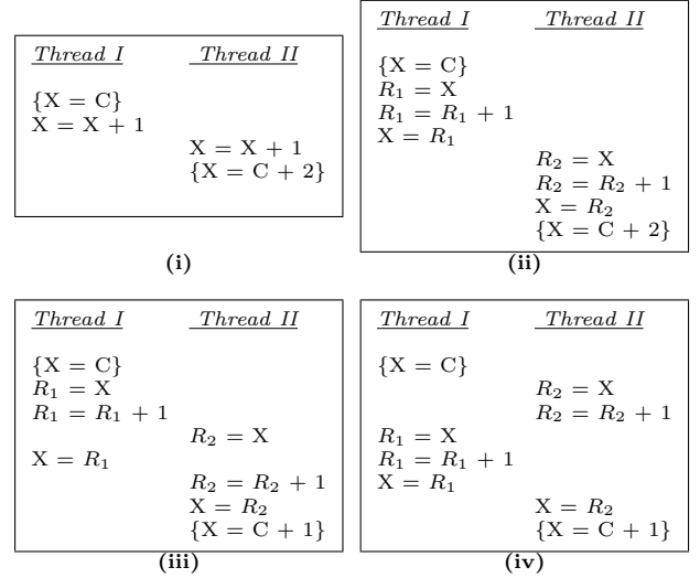
Figure 1: A datarace intuition example. (i) contains a program fragment with two threads such that each thread increments the value of a global variable X by 1. (ii) contains the same program as (i), but here we use two registers, R1 and R2 , to split X = X + 1 into three atomic operations. (iii) and (iv) contain the same program, but with a different thread interleaving. It is easy to see that the output of this execution is X = C + 1 and not the expected result X = C + 2 .
