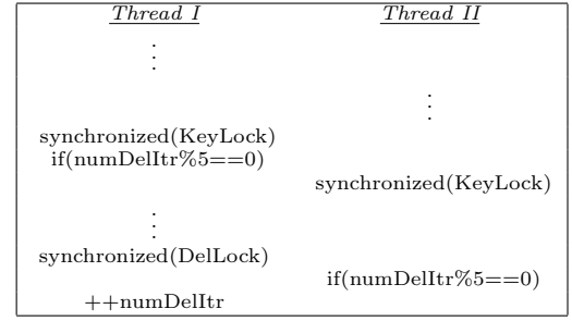
Figure 6: A witness that our technique generates for a datarace on variable numDelItr in the running example in Figure 4.
