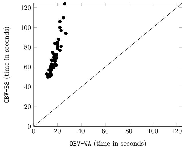
Fig. 5: Comparing OBV-WA to OBV-BS on industrial instances.
