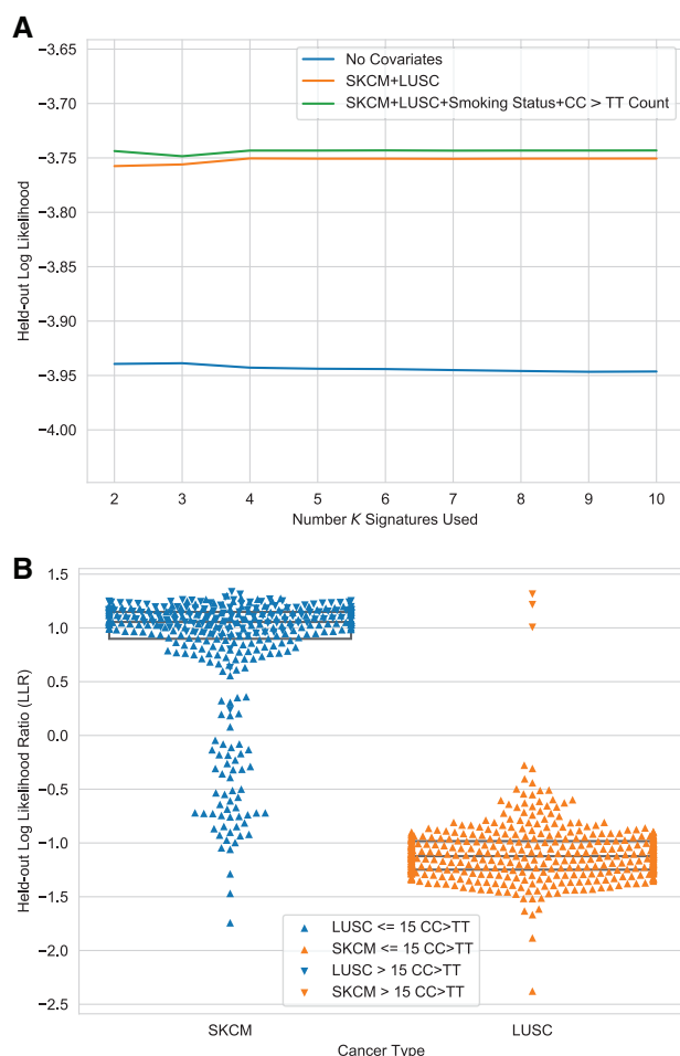
Fig. 4. (A) The held-out log-likelihood plot used for model selection to obtain K = 4 . (B) The log-likelihood ratio (LLR) of the cancer type covariate for tumors where LLR < 0 means the mutations of the tumor are more likely under LUSC and LLR > 0 means the mutations of the tumor are more likely under SKCM
