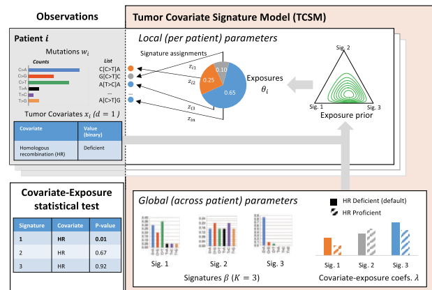
Fig. 1. Overview of the Tumor Covariate Signature Model (TCSM) with an illustrative example of d = 1 covariate and K = 3 signatures. For ease of illustration, the model shown is a simplified version of TCSM that does not model correlations between signatures. Given the observed mutations in a cohort of patients (top left), TCSM learns per patient exposures and assignments of each mutation to a signature (top right), and a global set of signatures and covariate-exposure coefficients (bottom right). The associations between covariates and exposures are then tested for statistical significance (bottom left). Parts of the design of the figure are inspired by Blei (2012) and Alexandrov et al. (2013b)
