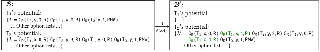
Fig. 5. Illustration of loSRA's WRITE step, as defined in Def. 5.9. Two read options O_R(T_1, x, 4, R) are added to the option list L' of thread T_2 in \mathcal{B}' , constructed from the list L of T_2 and justified by the list \hat{L} of T_1 in \mathcal{B} . Observe that \hat{L} = L_1 \cdot L_2 , L = L_0 \cdot L_1 \cdot L_2 and L' = L_0 \cdot O_R(T_1, x, 4, R) \cdot L_1 \cdot O_R(T_1, x, 4, R) \cdot L_2 , where L_0 = O_R(T_1, x, 0, R) , L_1 = O_R(T_2, y, 3, R) \ O_R(T_1, y, 0, R) and L_2 = O_R(T_2, y, 1, RMW) .
