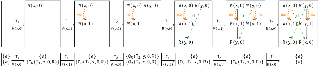
Fig. 4. Illustration of runs of opSRA (top) and loSRA (bottom) for the SB program (Ex. 3.3). In opSRA’s states (execution graphs), events of T_1 are on the left and of T_2 on the right. In loSRA’s states (a potential for each thread), the potential of T_1 is at the top and of T_2 at the bottom. In this simple example, all option lists consist of at most one option and all potentials are singletons.
