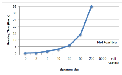
Figure 5: Running times for Dimension reduction
