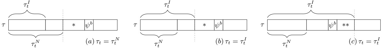
Figure 3: Cases in the proof of Lemma 9. * all actions by t are transactional; ** all actions by t come from a single transaction, started before or by \psi^b
